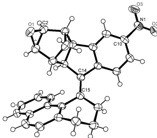
Figure 5. ORTEP representation of compound 12 . Thermal ellipsoids are set at 50% probability.
